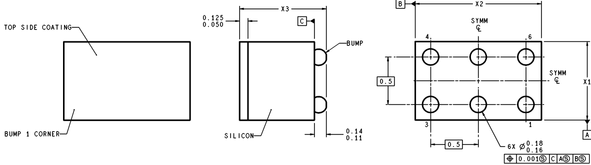
DIMENSIONS ARE IN MILLIMETERS
