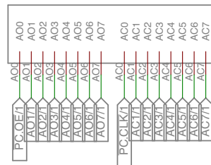
ABus Control
