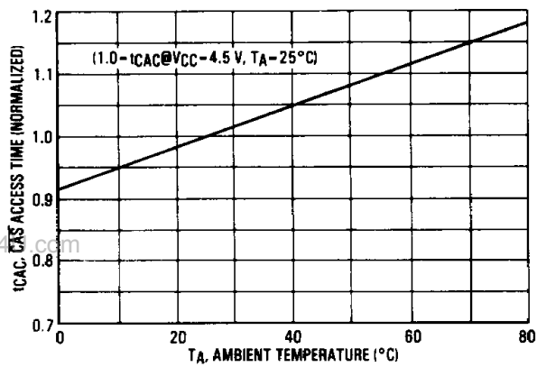
FIGURE 5 - \overline{CAS} ACCESS TIME versus AMBIENT TEMPERATURE
