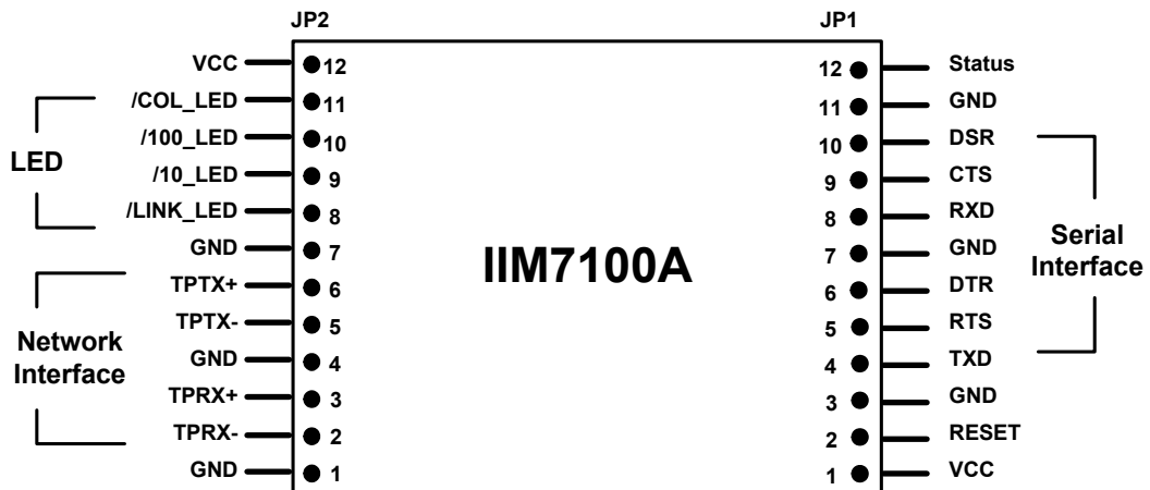
[IIM7100A Module Pin Assignment]
